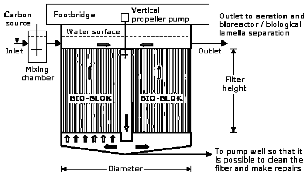
Principle drawing
